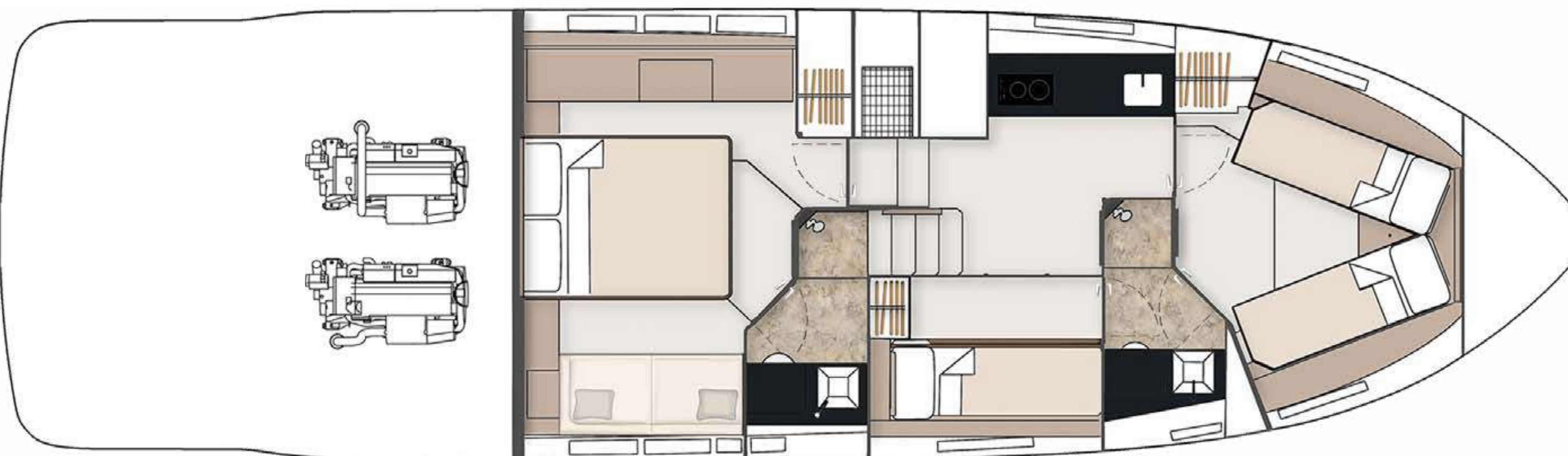
THREE CABIN
